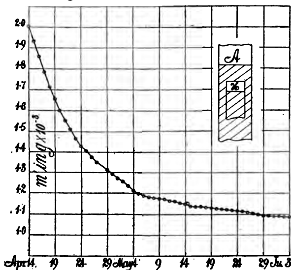
FIG. 10.—Chart showing loss of mass of gas in diver in lapse of days. Diffusion of hydrogen into air.
